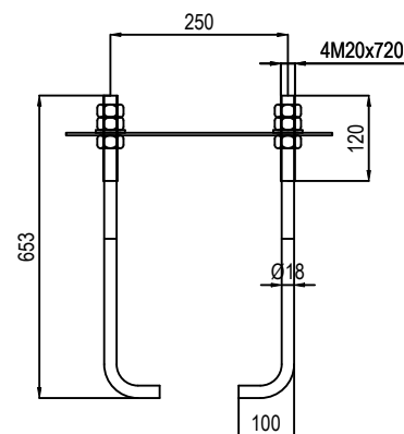
ANCHOR BOLT
