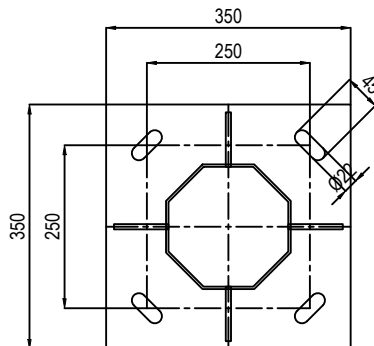
BASE PLATE #14x350x350
