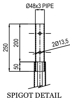
SPIGOT DETAIL
