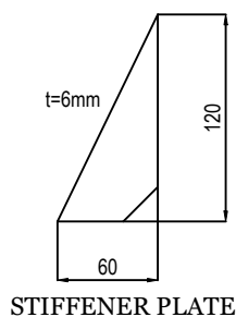
STIFFENER PLATE
