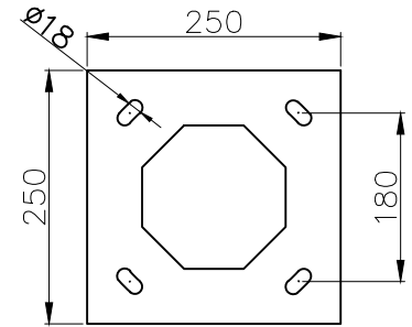
BASE PLATE # 10 mm x 250x 250
